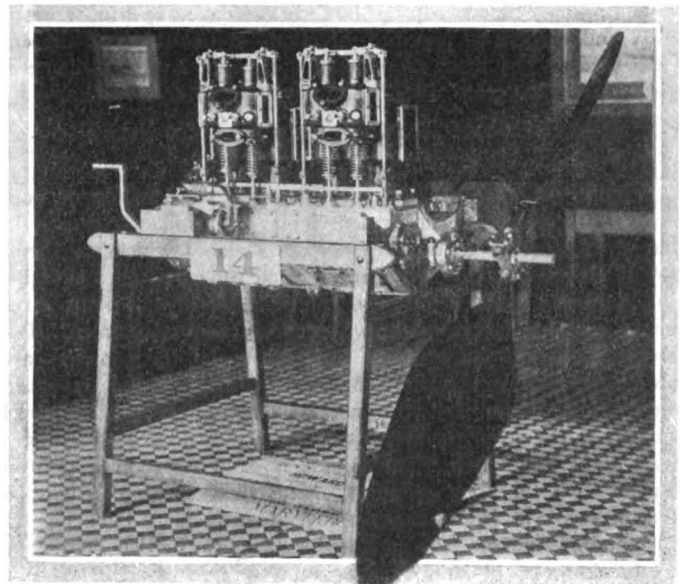
Four-Cylinder, 50-HP. Metallurgique Aero Engine.
